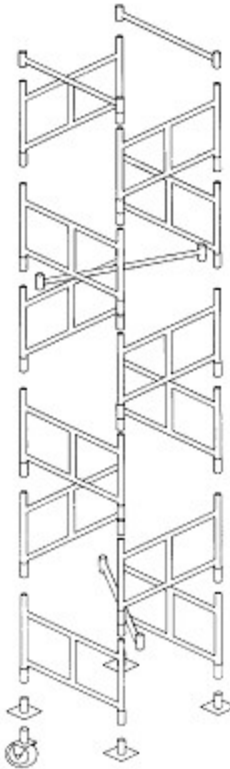
Standard Tower Kit (with optional castor)
